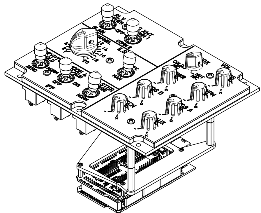
-1 ISO SCALE 1:2
